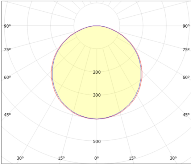
cd 1170 lm — C0/C180 — C90/C270
