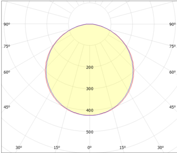
cd 1230 lm — C0/C180 — C90/C270
