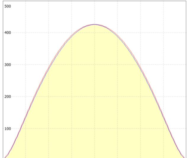
cd 1230 lm — C0/C180 — C90/C270
